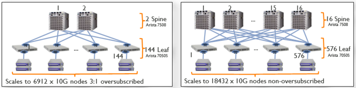
Arista Leaf-Spine Two-Tier Network Architecture
